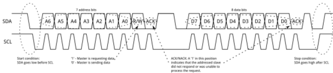
Figure 3.9: Clock cycle
