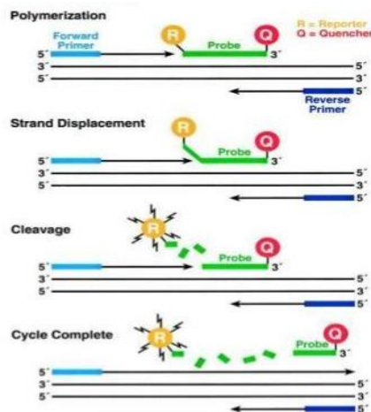
Figure 5.5: Functionality of the TaqMan probe and source of the fluorescence.
