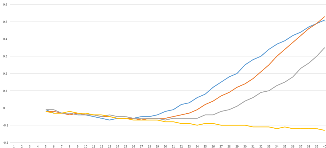
Figure 7.3: Experimental data that should be replicated by new PCR machine. The four curves, blue, orange, gray, and yellow, are the samples containing 10^7 , 10^6 , 10^5 , and the control respectively.
