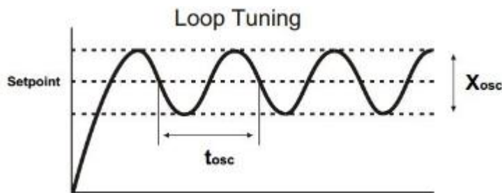
Figure 3.15: Oscillations used for loop tuning.
