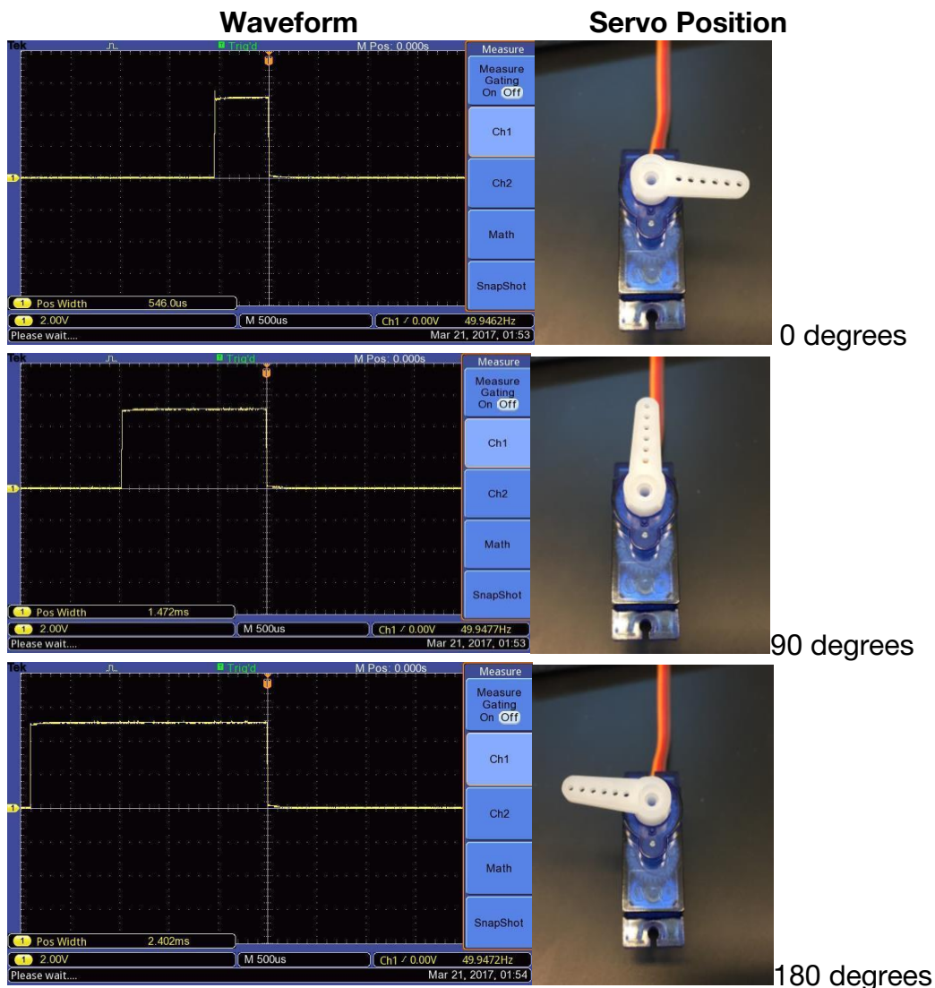
Figure 3.21: The servo positions resulting from various PWM.
