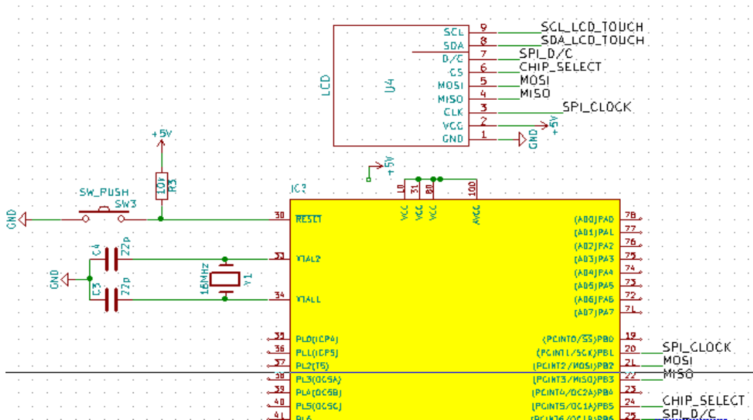
Figure 5.24: Schematic interface
