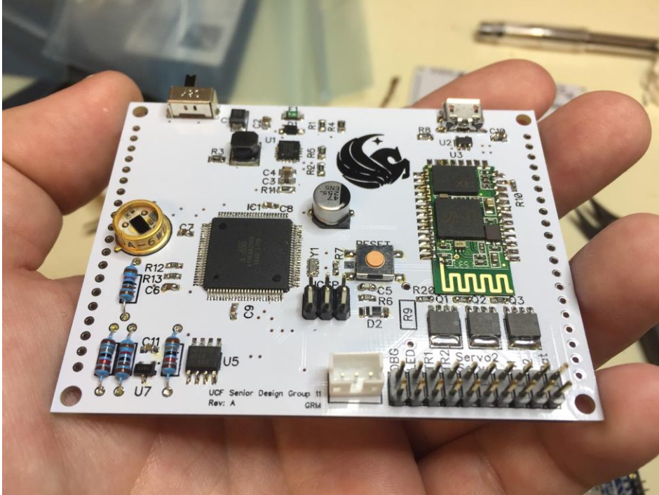
Figure 6.5: PCB after population and soldering of the electronic components.
