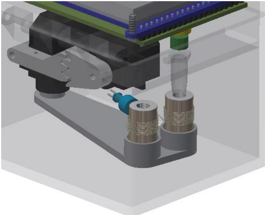
Figure 5.20: The two temperature control modes of the device, top: cooling mode, bottom: heating mode.
