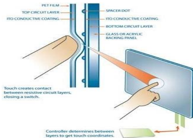
Figure 3.26: This figure depicts the resistive touch screen. Its operation will be used similarly for the touchscreen of our Portable PCR machine.
