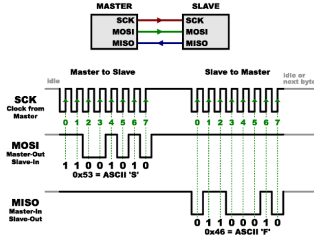
Figure 3.11: Clock cycle
