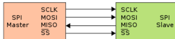
Figure 3.10: SPI Connections
