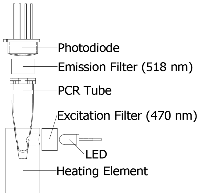
Figure 5.6: Optical components of the qPCR device.
