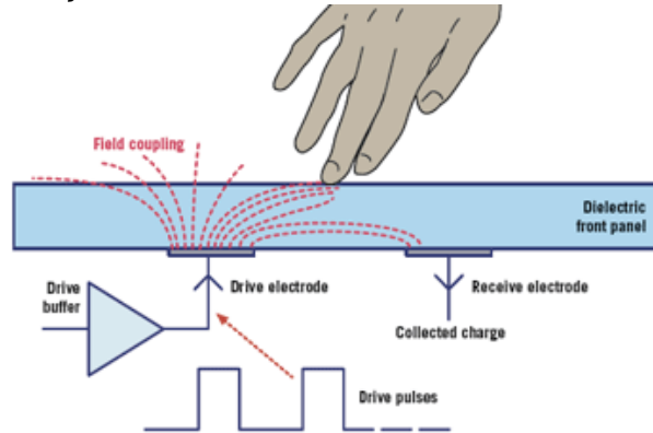
Figure 3.25: Projected capacitive touchscreen. This figure recognizes the capacitive touch screen as explained from above.
