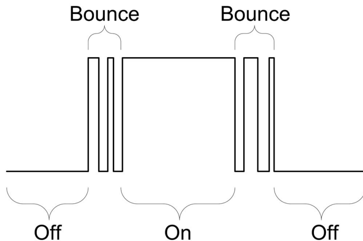
Figure 5.18: waveforms caused by switch bouncing.
