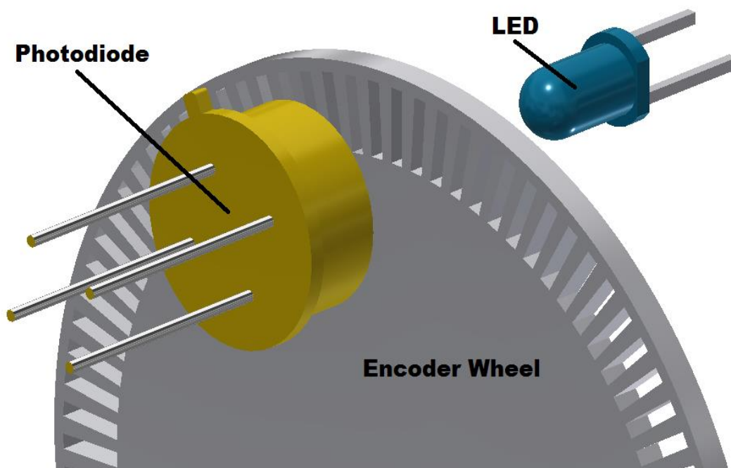
Figure 5.22: Detail of the rotary encoder used in a servo motor, light from the LED is passed through slots on the encoder wheel and is read by the photodiode. The pulses of light seen by the photodiode allow for the controller to determine the position of the encoder wheel.
