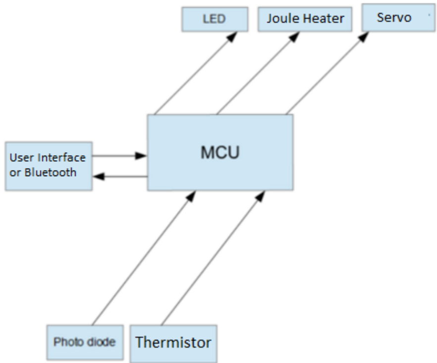
Figure 5.8: Block diagram showing the inputs and outputs the MCU is responsible for.
