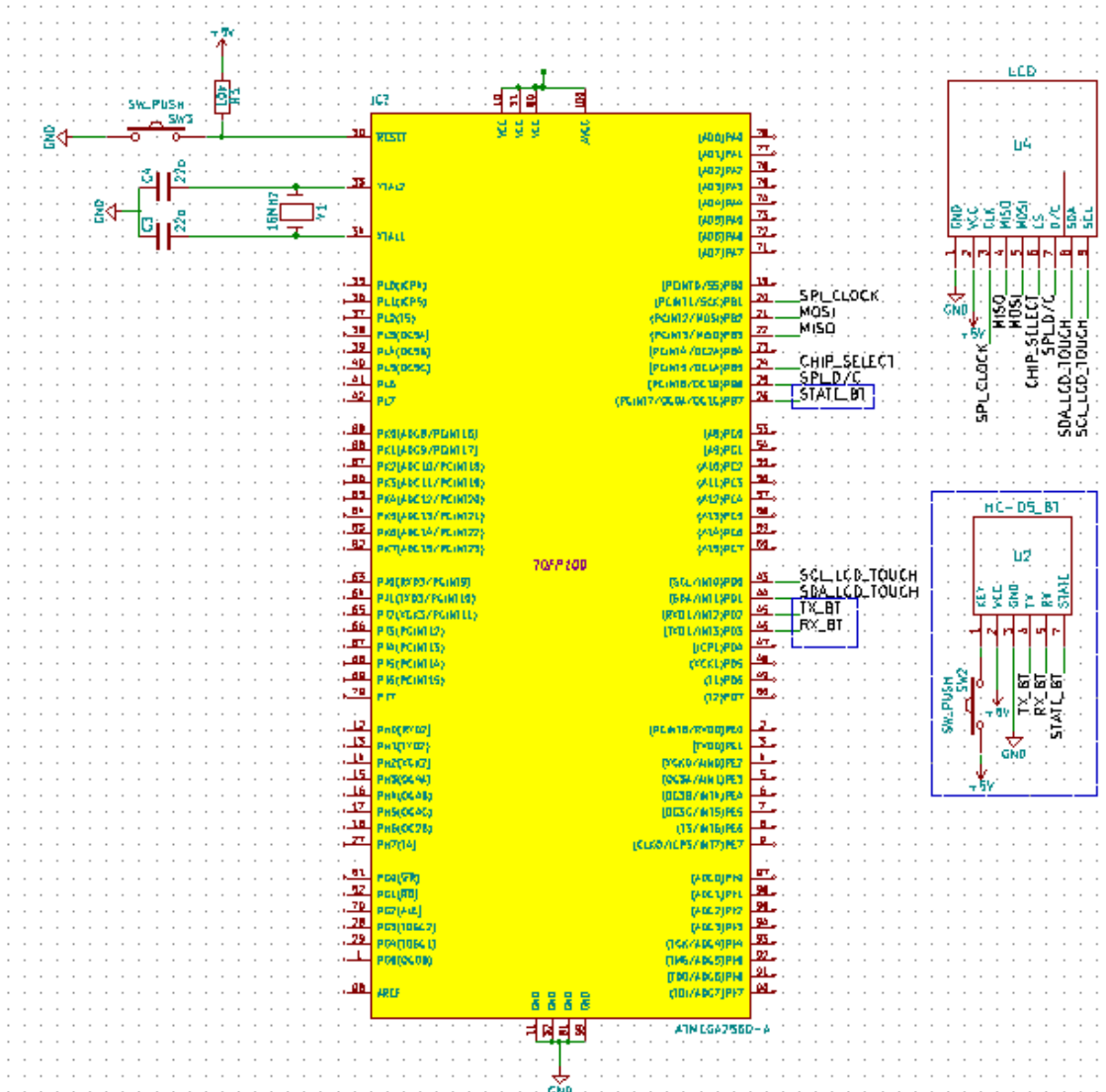
Figure 5.23: Interface Schematic
