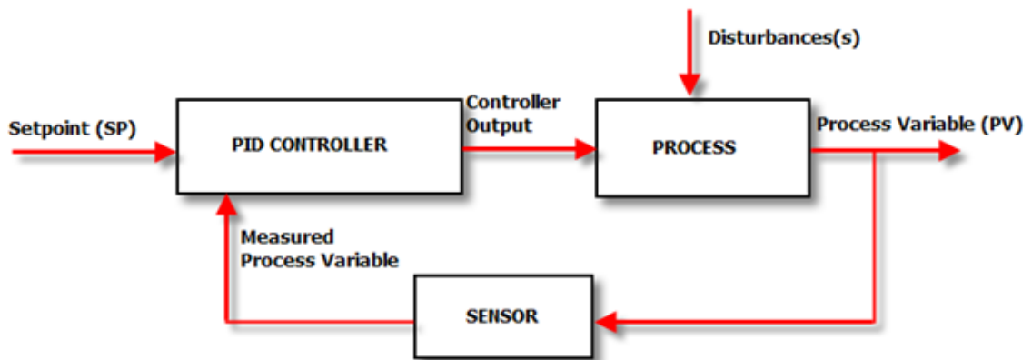
Figure 3.12: This diagram shows the block diagram for a typical PID controller system.
