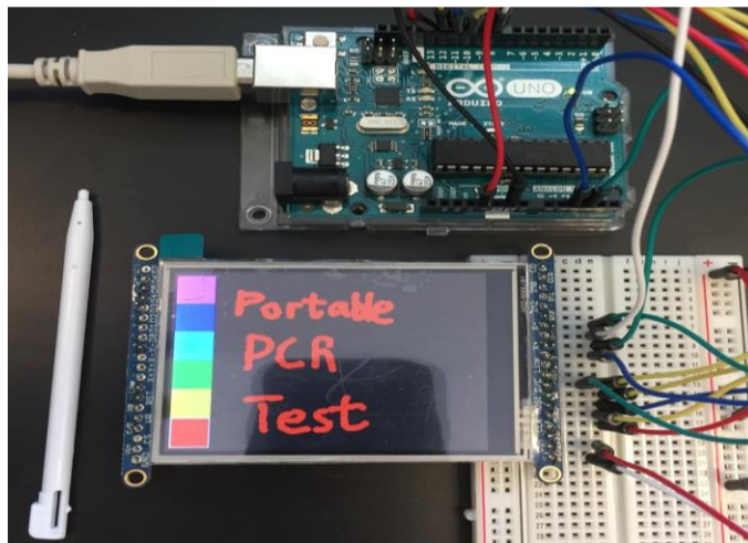
Figure 5.25: Breadboard test of the LCD, touchscreen, and Microcontroller.
