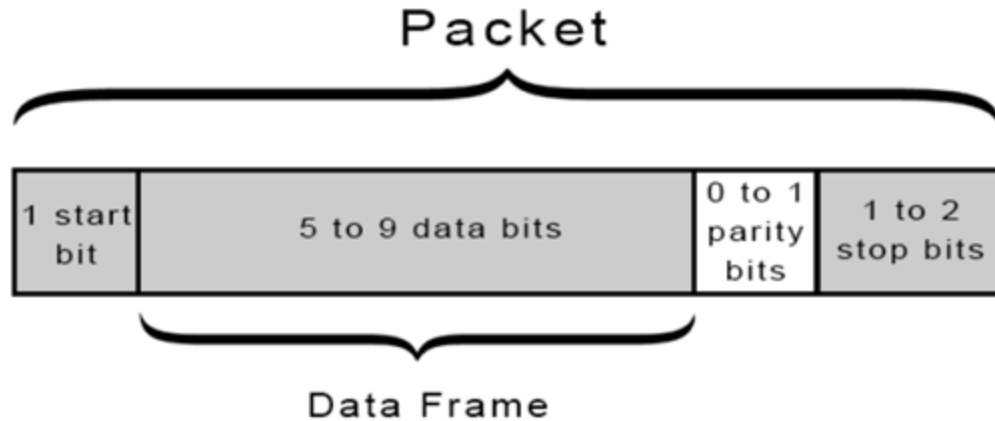
Figure 3.17: Breakdown of a packet sent by a UART, showing the bit fields and data frame location.
