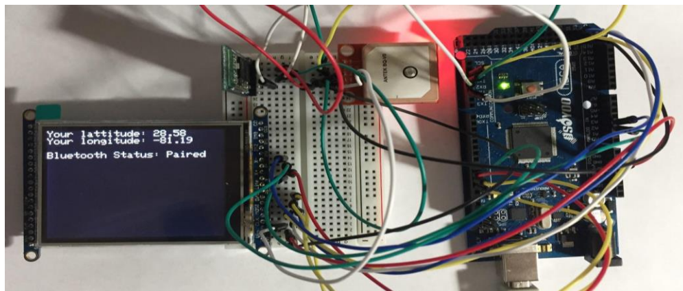
Figure 5.26: Breadboard testing of several major components simultaneously.
