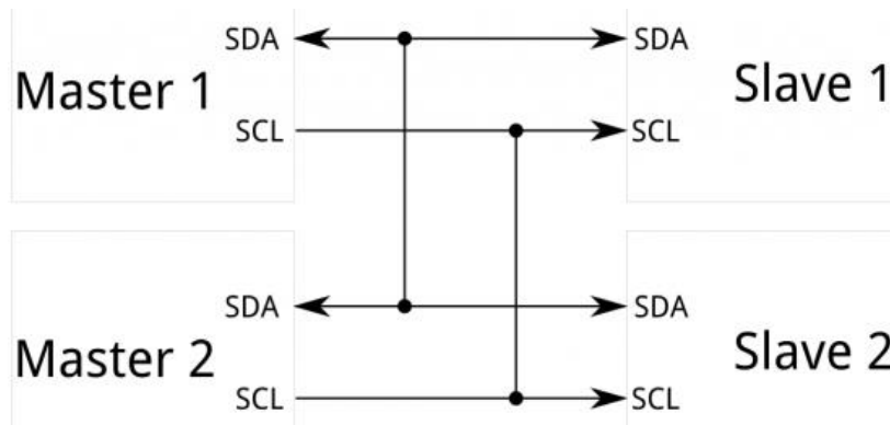
Figure 3.8: I2C Connection example
