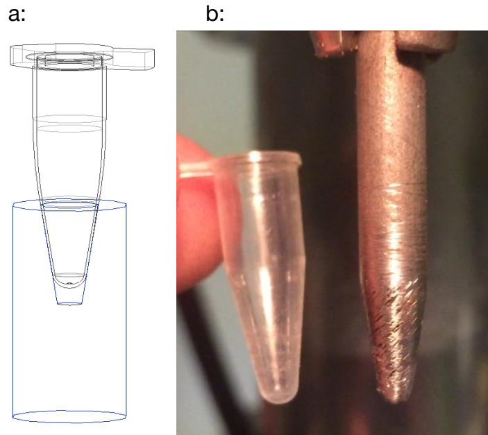
Figure 6.1: a: Detail of the heating element and PCR tube contact. b: Shaping tool used to bore conical hole in the heating element.
