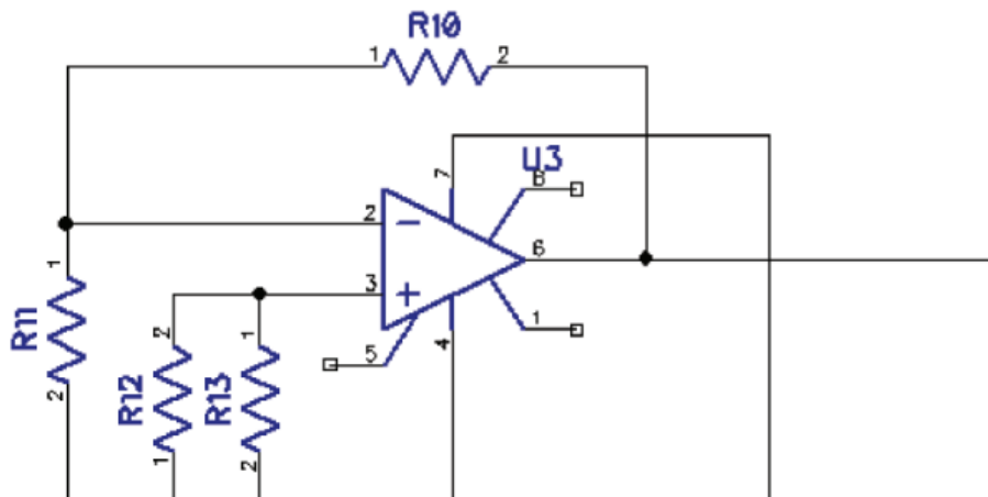
Figure 3.27: Use of MAX406 difference amplifier
