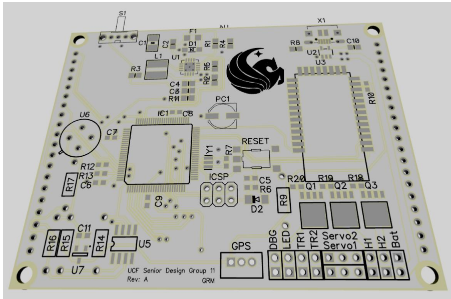
Figure 6.3: PCB layout as designed in DipTrace
