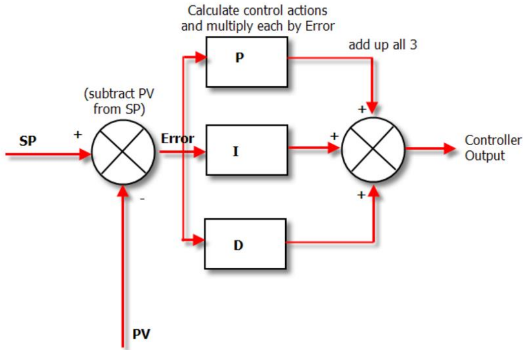
Figure 3.13: Block diagram of a PID controller system.
