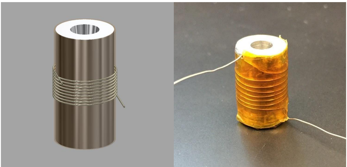
Figure 5.1: Left: The heating element as designed in Inventor. Right: The heating element as constructed using NiCr wire.
