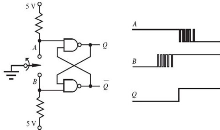
Figure 5.19: schematic and waveforms of a debouncing circuit.
