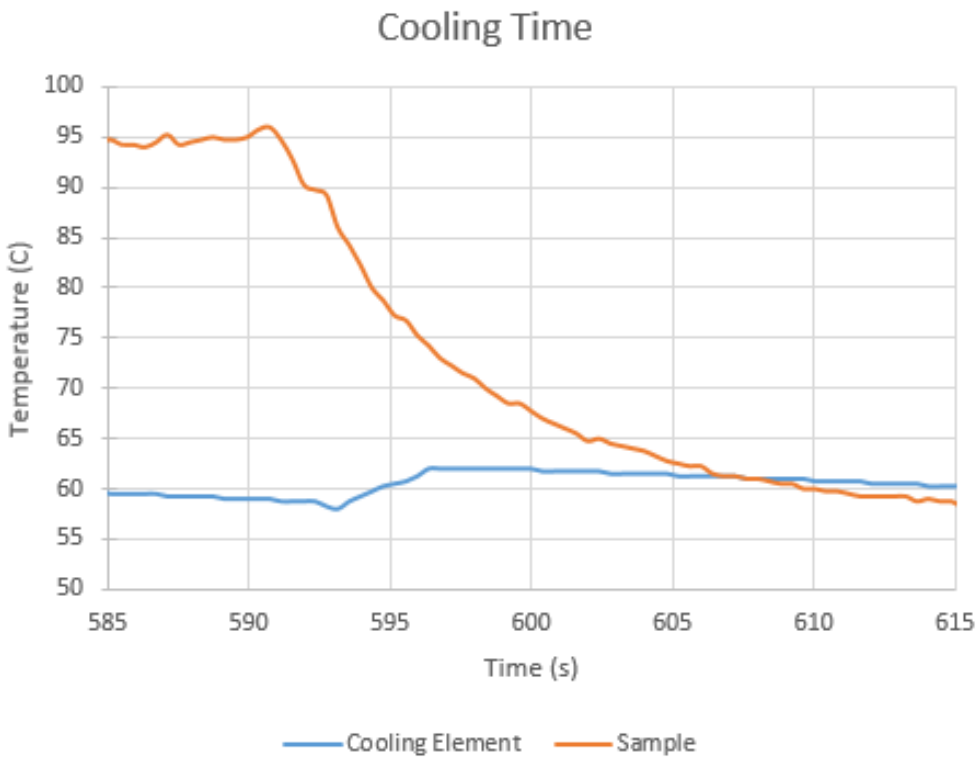
Figure 7.1: Heating and cooling test thermal plots used to determine heating and cooling time.
