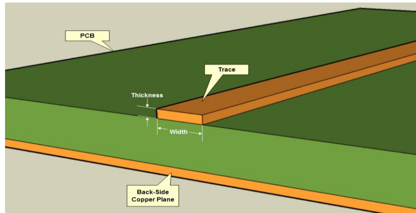
Figure 4.1: Structure of FR-4 fiberglass circuit board.
