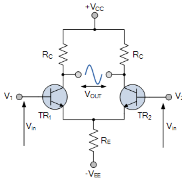
Figure 3.24: Difference amplifier using transistors
