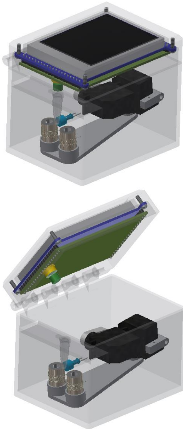
Figure 5.21: Demonstration of the opening of the device. Top: the device in its closed state, bottom: the device with its lid open, allowing insertion of the PCR tube. The green board is the main PCB.
