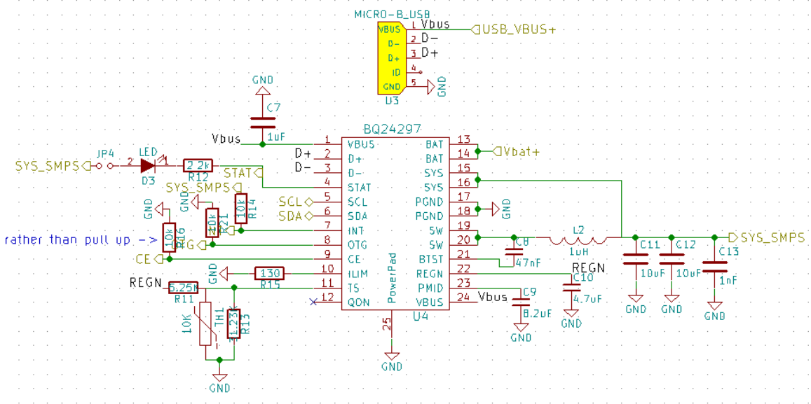
Figure 5.17: Schematic of a low parts count charger
